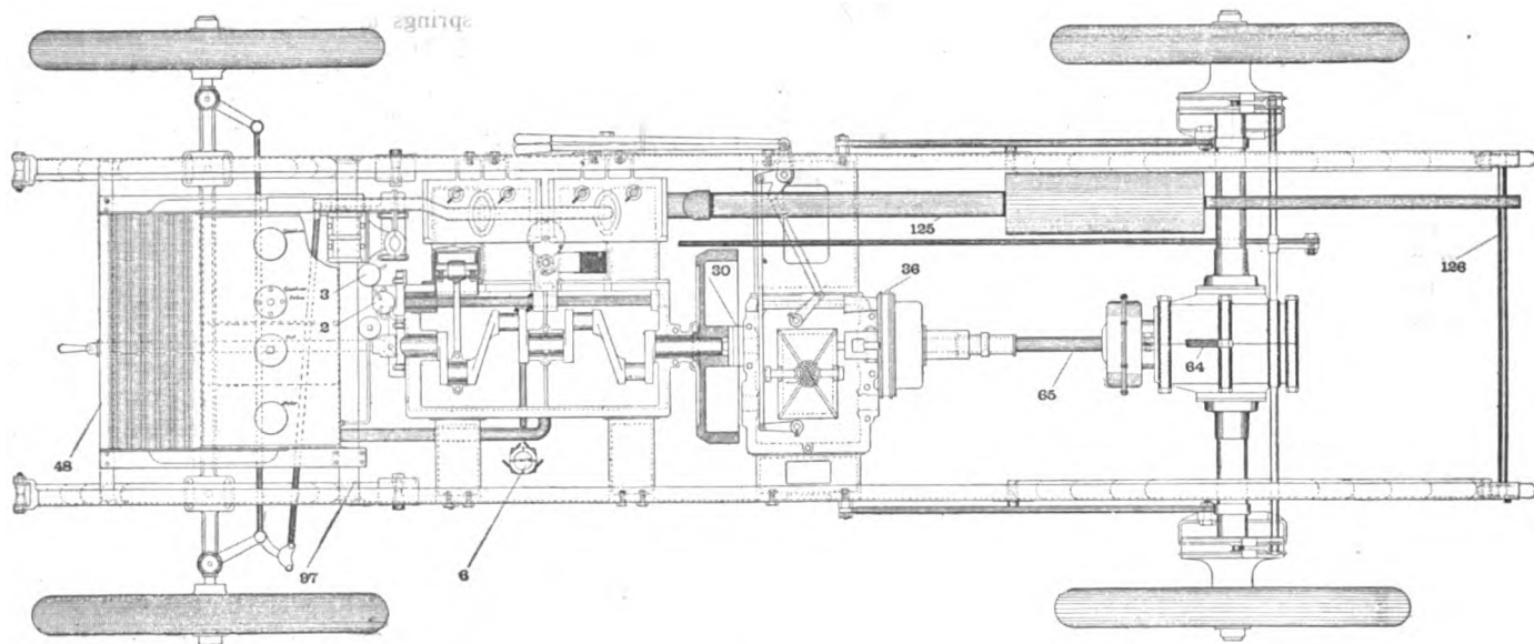
PLAN OF NEW WINTON TOURING CAR. SHOWING DISPOSITION OF QUADRUPLE ENGINE UNDER FOOTBOARD.
